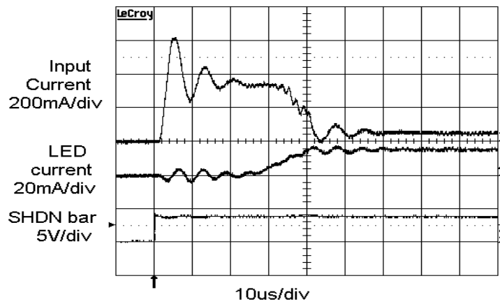
Figure 12. Enable Power-Up Waveforms
