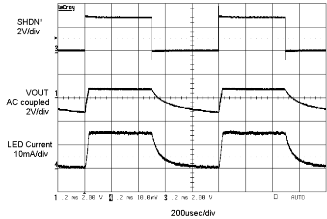
Figure 11. PWM on SHDN Pin at 1 kHz
