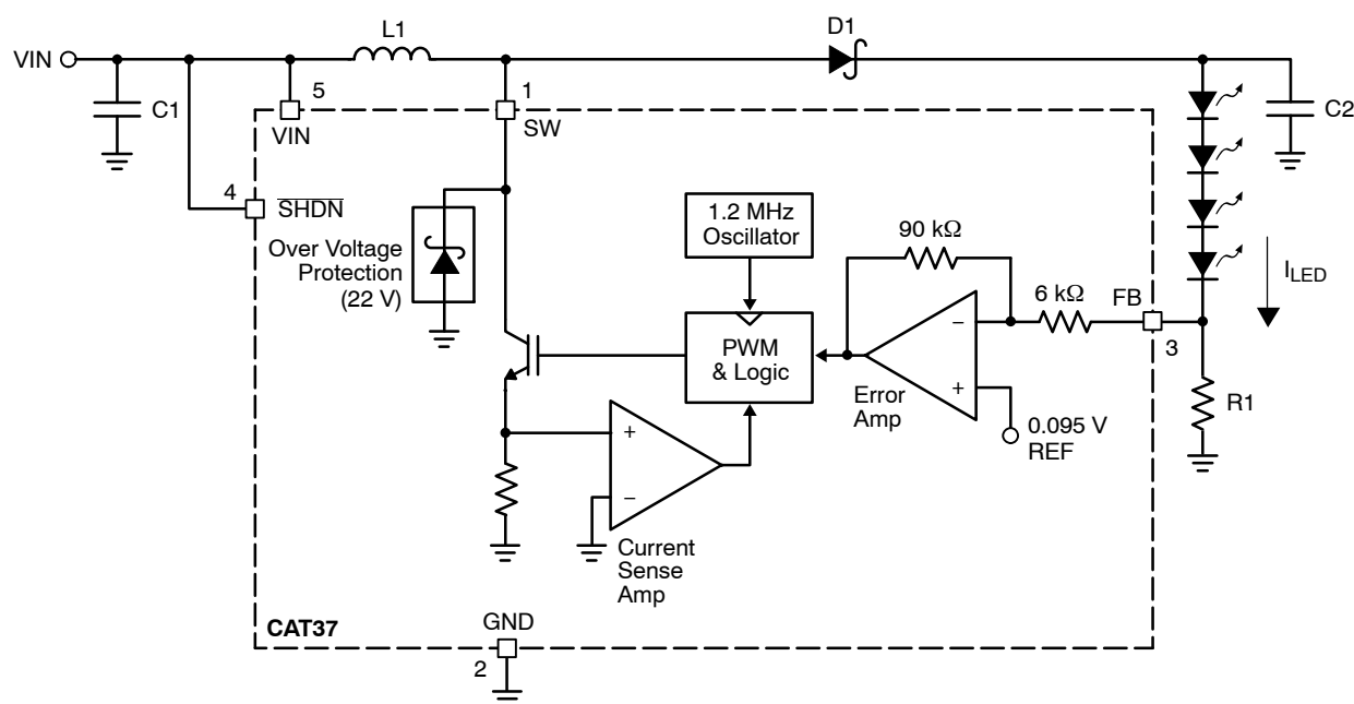
Figure 13. CAT37 Block Diagram
